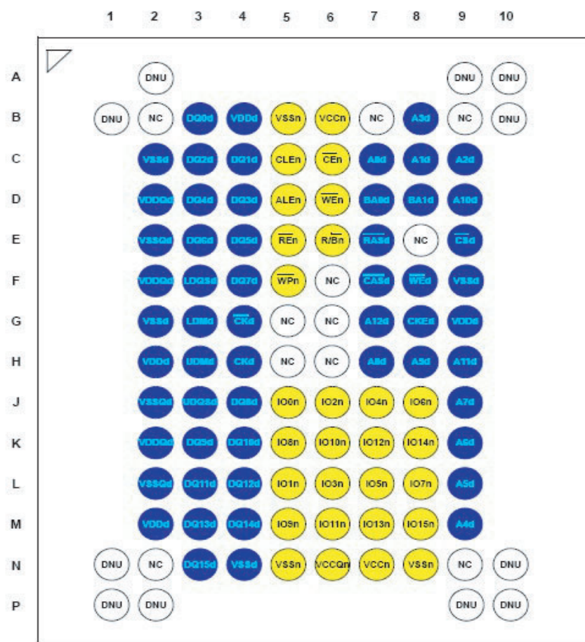
107 FBGA: Top View (Ball Down)
